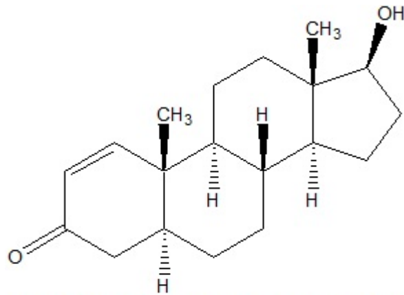
17beta-Hydroxy-5alpha-androst-1-en-3-one
